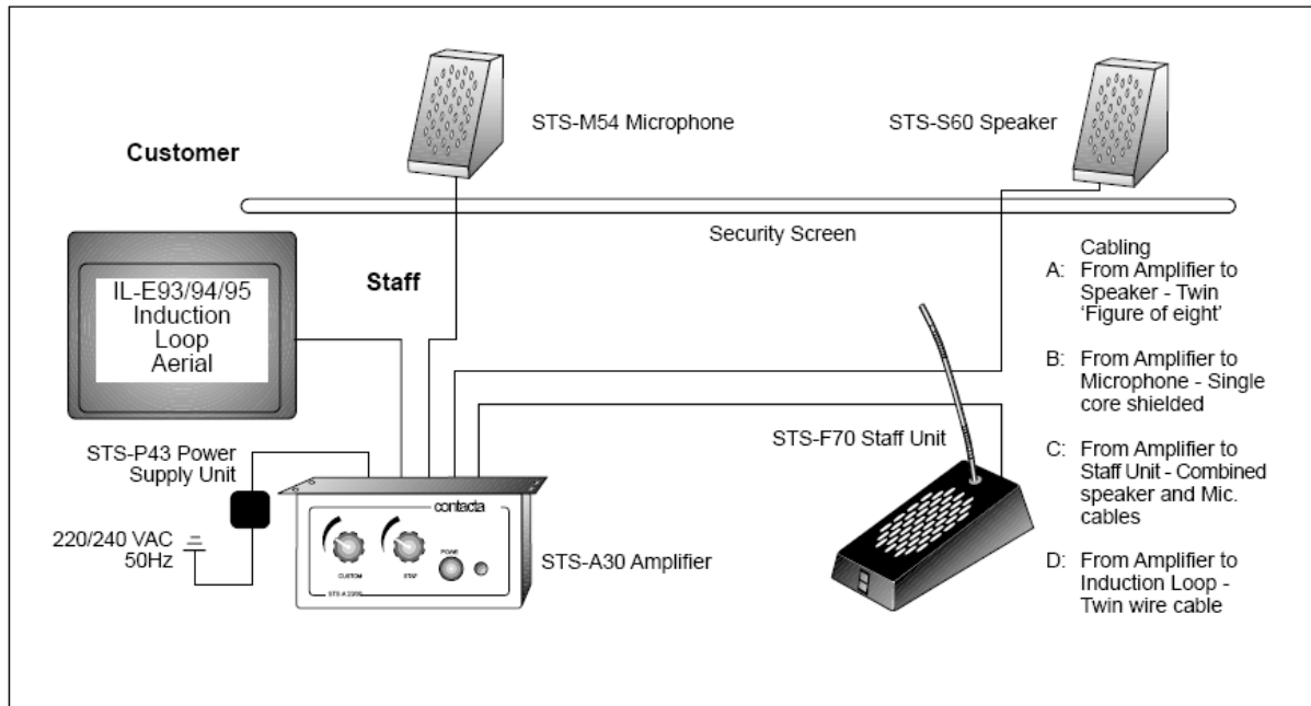
Typical system arrangement with surface mounting customer speaker & microphone
